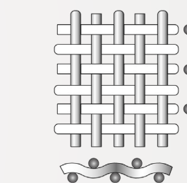
Square opening plain weave
