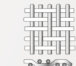
Square opening twill weave
